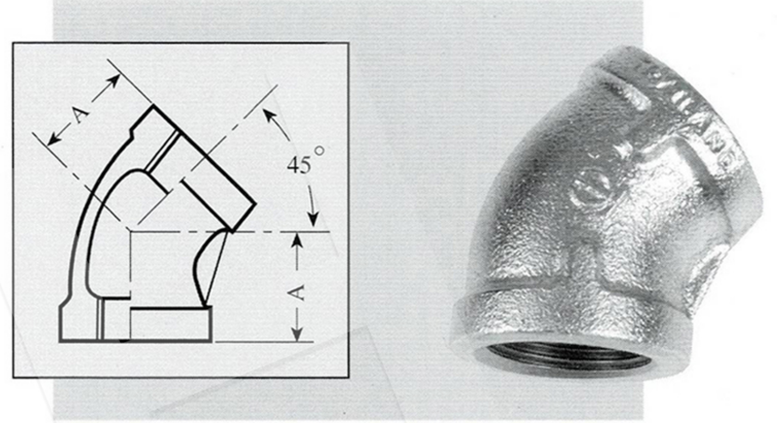
FIG.122 Elbow, 45°, Banded (BL45°)
